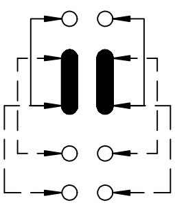
SCHEMATIC (SHORTING)
