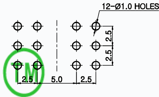
PCB Dimension
