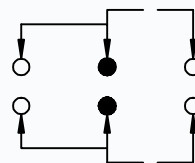
SCHEMATIC (NON-SHORTING)
