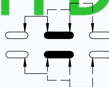
SCHEMATIC (NON-SHORTING)
