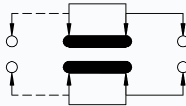
SCHMATIC (NON-SHORTING)
